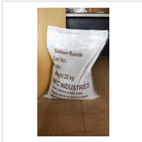
Sodium Fluoride
