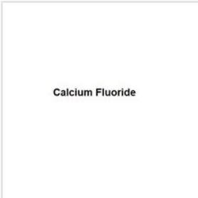
Calcium Fluoride
